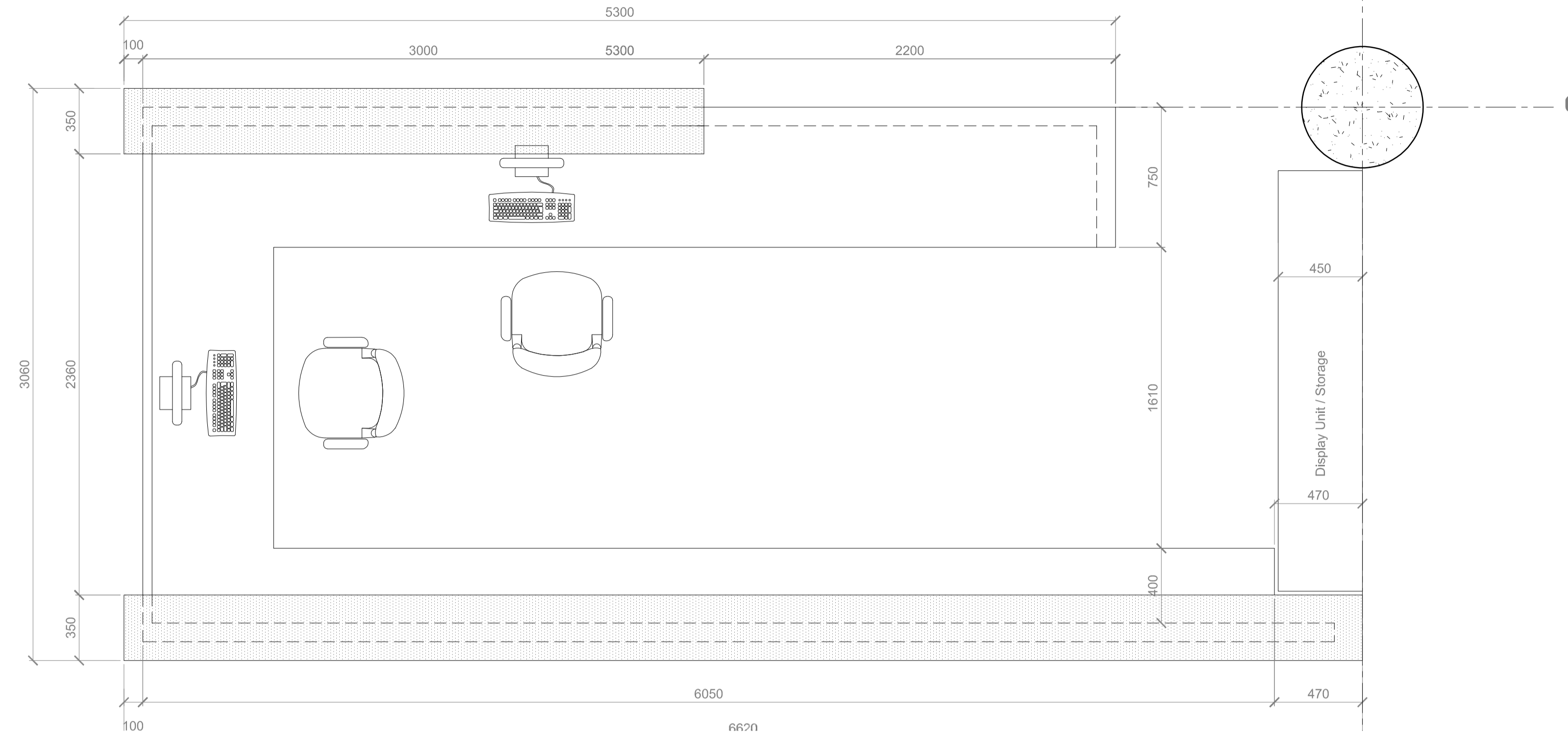
2 Plan - High Counter Scale 1:20
